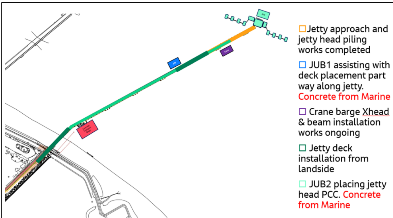
Plate 1-5: Example landside and marine construction sequence
