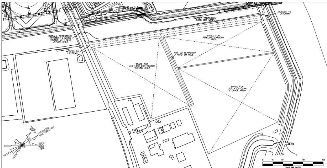
Plate 1-4: Indicative arrangement of Work No. 9
